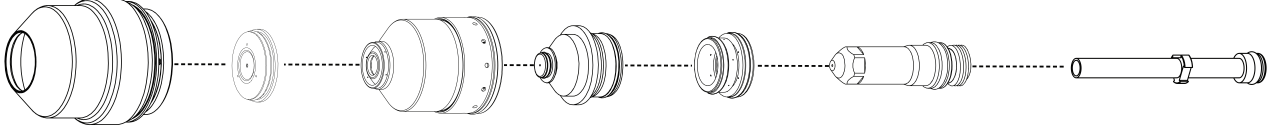
HYPERTHERM HYPERFORMANCE PLASMA HSD130XD - HAFİF ÇELİK
