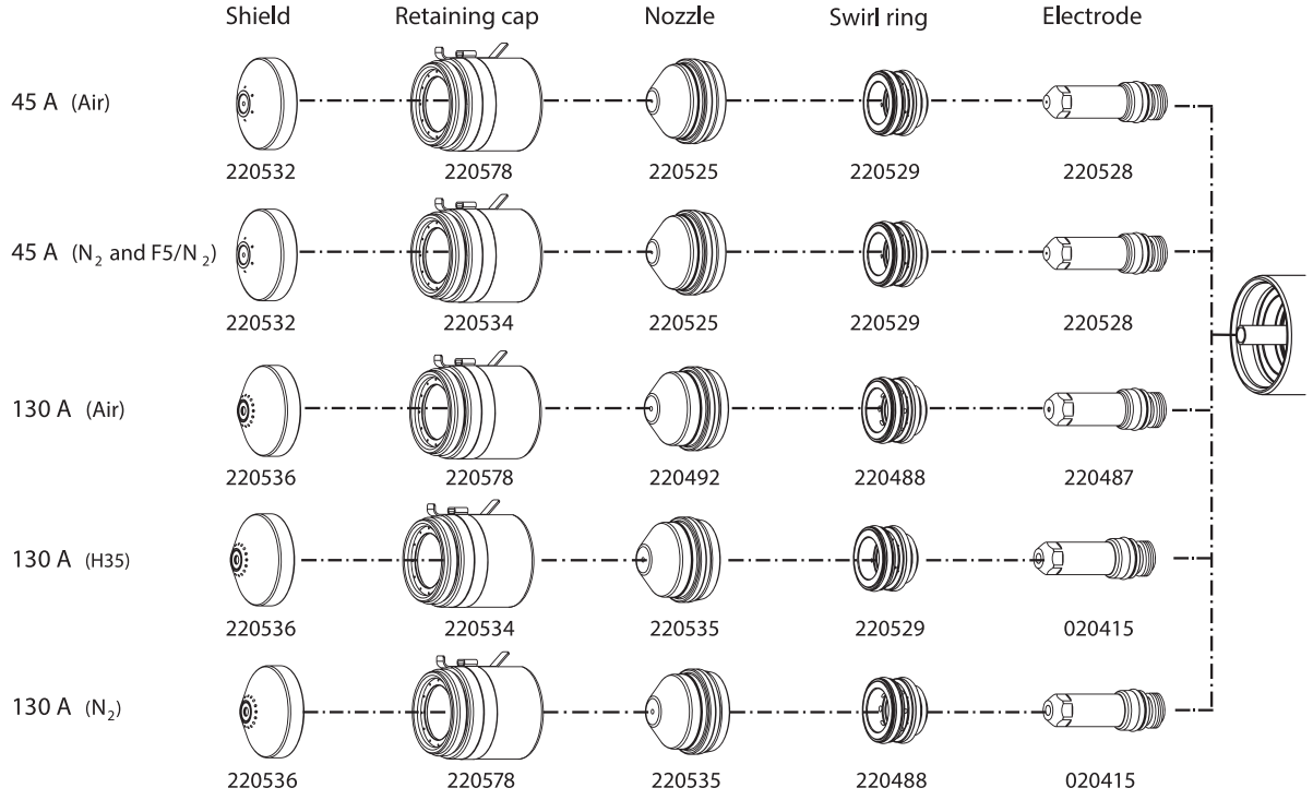
HYPERTHERM HYPERFORMANCE PLASMA HSD130 - STAINLESS STEEL
