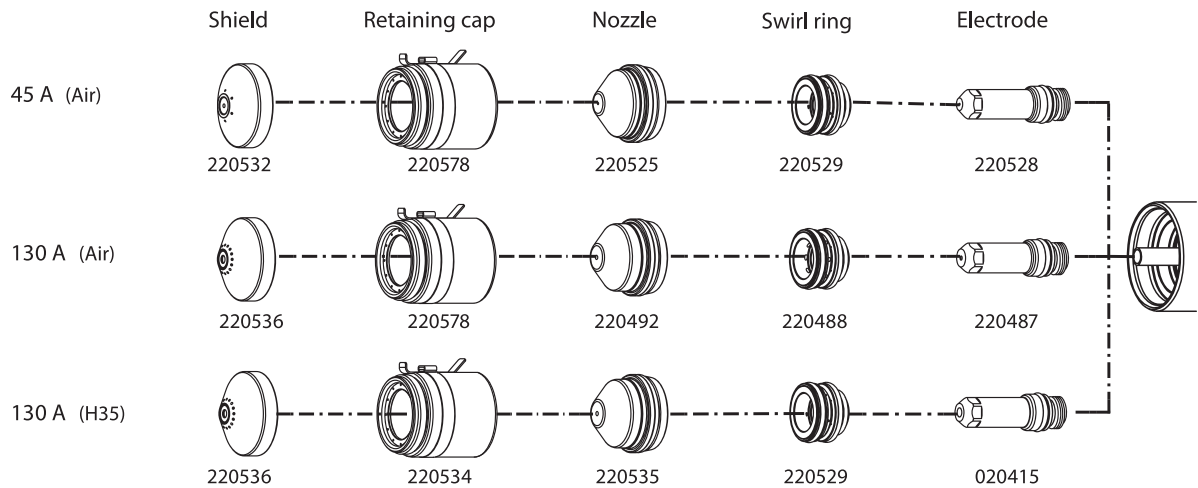
HYPERTHERM HYPERFORMANCE PLASMA HSD130 - ALÜMİNYUM
