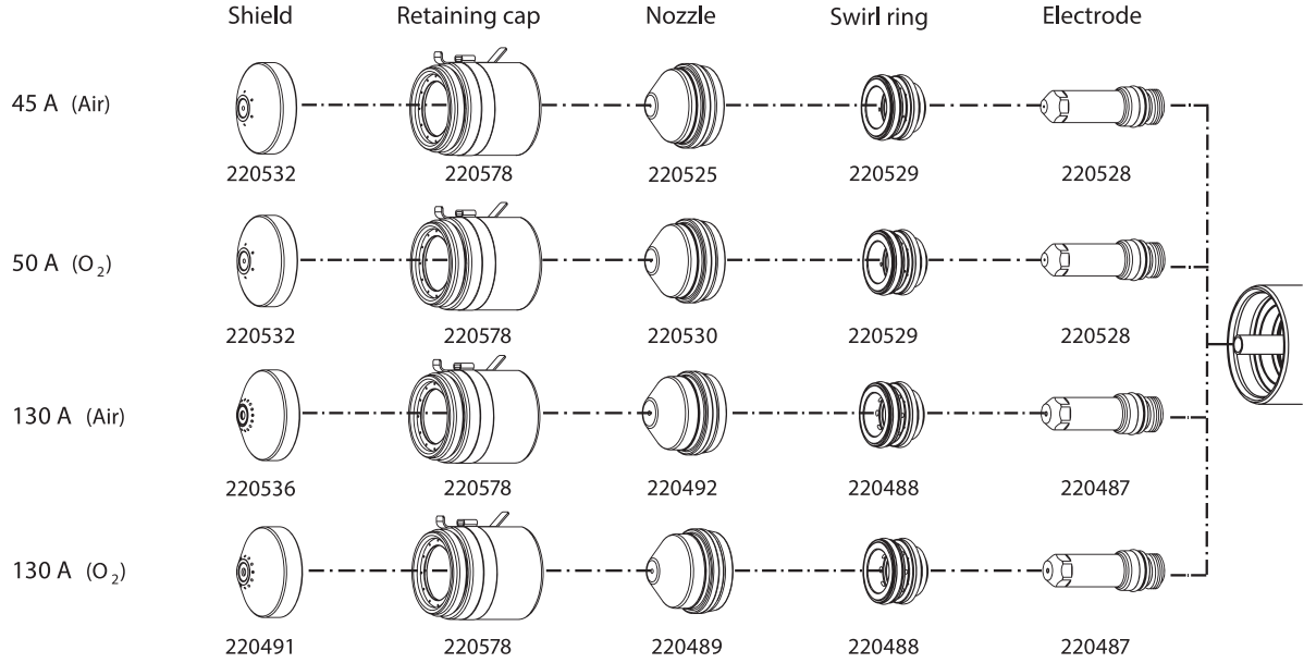
HYPERTHERM HYPERFORMANCE PLASMA HSD130 - HAFİF ÇELİK
